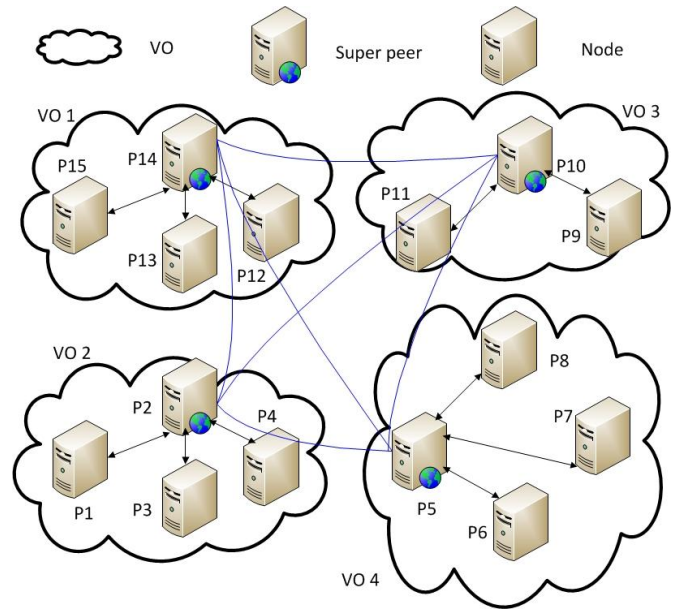
Fig. 1. the routine of node grouping
